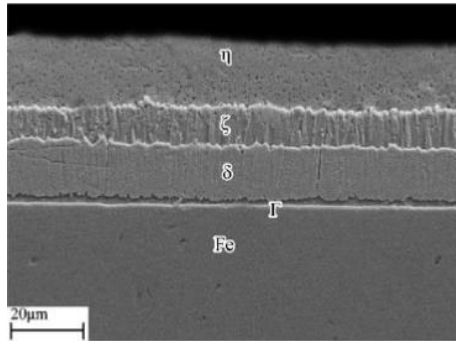
Figura 2. Fases gamma, delta y zeta (Rico, Y. Carrasquero, E. 2017)
