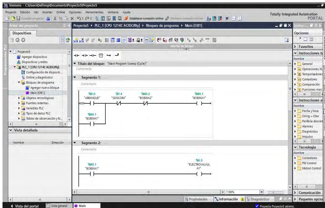
Figura No. 8 TIA portal v13 ladder
